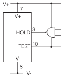
Driving HOLD from external logic.
